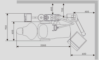
Exteranal floor-box installation sketch map
