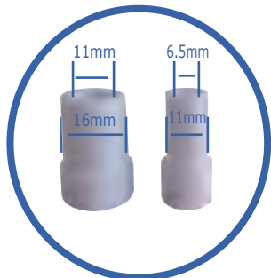
• 11-10024 Connector 11x16 100pcs/bag,50bags/ctn
